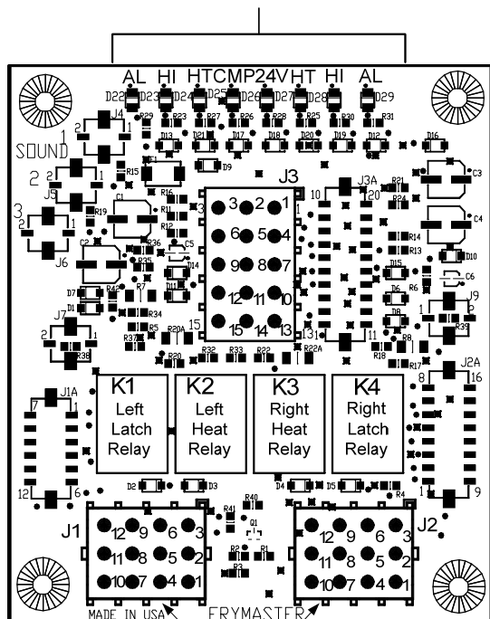
Diagnostic LEDs
